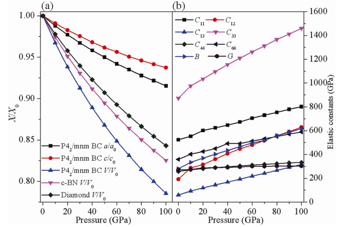
Fig. 2—(a) Lattice parameters a/a_0 , and c/c_0 compression as functions of pressure for P4 2 /mm-BC, and primitive cell volume V/V_0 for P4 2 /mm-BC, c-BN, and diamond and (b) Elastic constants of P4 2 /mm-BC as a function of pressure
