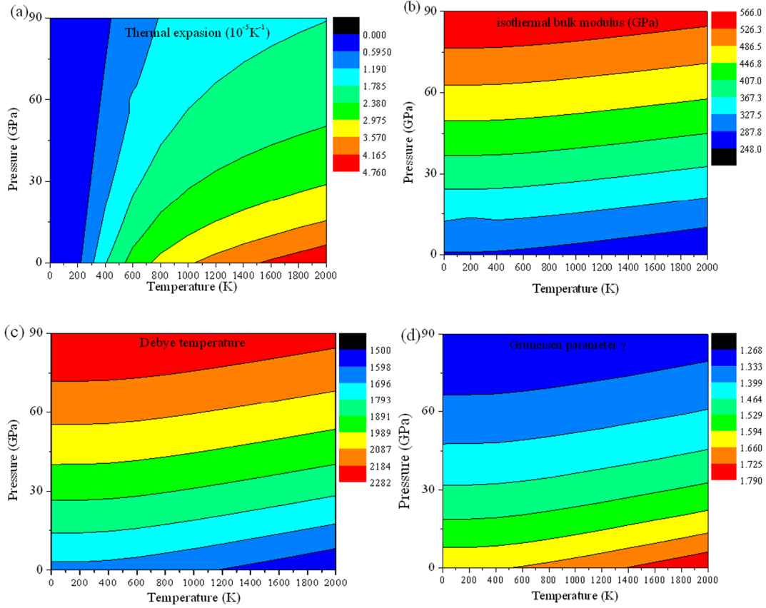
Fig. 6—(a) Two-dimensional contour plots of thermal expansion, (b) isothermal bulk modulus, (c) Debye temperature and (d) Grüneisen parameter versus pressure and temperature for P4_2/mnm -BC
