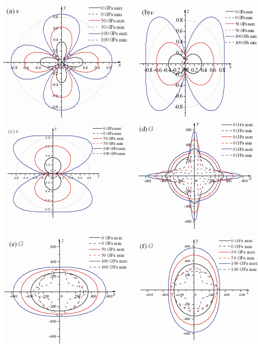
Fig. 3—2D representation of Poisson's ratio in the (a) xy plane, (b) xz plane and (c) yz plane for P4_2/mnm -BC. 2D representation of shear modulus in the (d) xy plane, (e) xz plane and (f) yz plane for P4_2/mnm -BC
