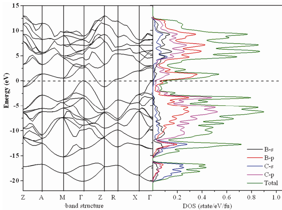
Fig. 5—Electronic band structure and density of state for the P4_2/mnm -BC at 0 GPa
