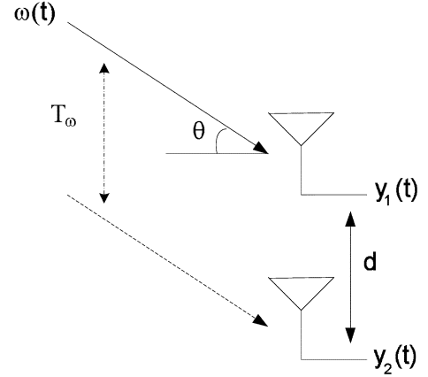
Fig. 2. Schematic of wavefront impinging on an antenna array. Under the narrowband assumption the antenna outputs y_1(t) and y_2(t) are identical except for a phase shift.
